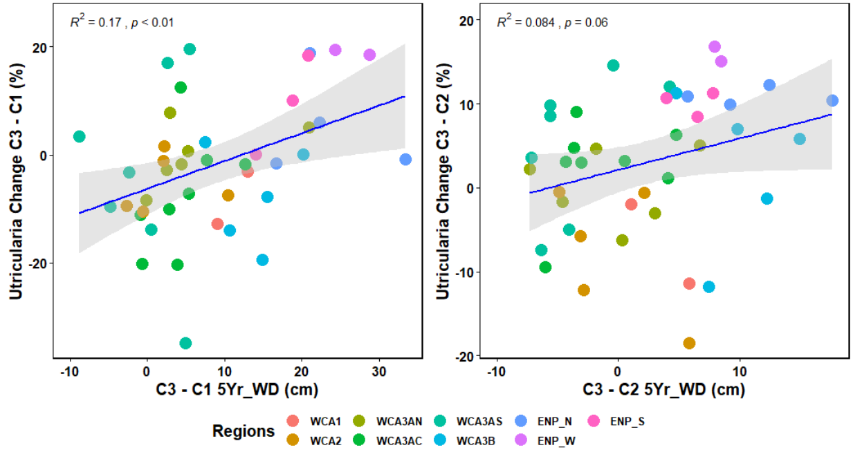
Figure 12: Change in 5-year average mean water level vs change in relative cover of bladderworts ( Utricularia spp.) in the 47 PSUs sampled over four years (Year 1-4; 2020-2024) of Cycle-3.
