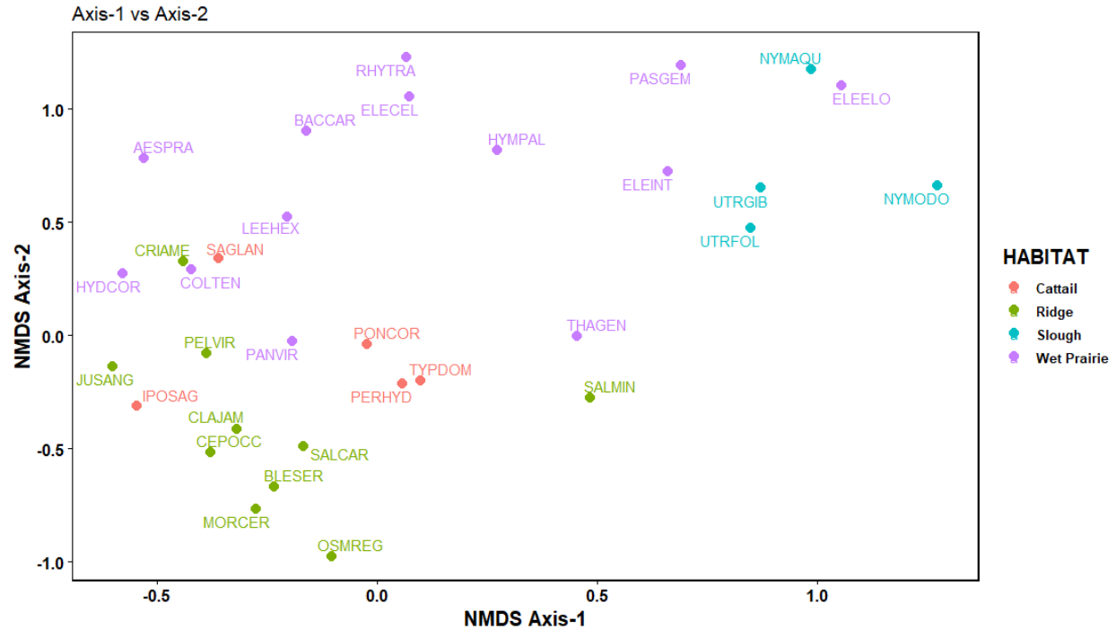
Figure 14: Distribution of major ridge-slough plant species in ordination space. It is noted that coherent clustering of species occurs by community type, which indicates relatively strong fidelity of species to their associated communities across the landscape. Species names are given in Appendix 2.
