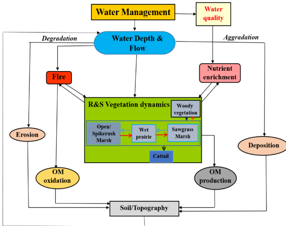
Figure 2: Conceptual model showing the relationships among causal factors such as soil microtopography, water regimes and disturbances (fire and nutrient enrichment) and vegetation dynamics within R&S landscape (Modified from Ross et al. (2006)).
