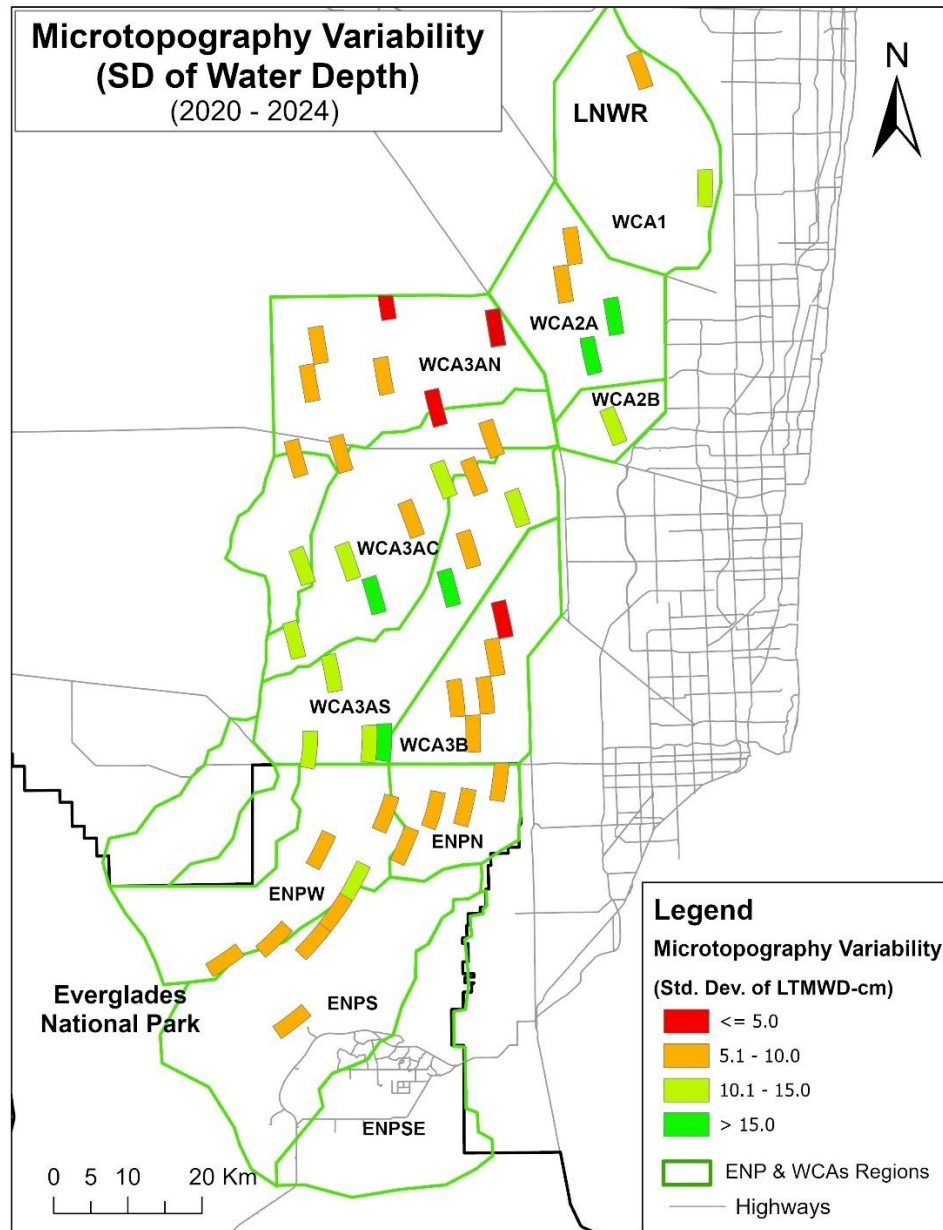
Figure 8: Spatial patterns of elevation variance across historic ridge-slough landscape represented by 47 PSUs sampled over four years (Year 1-4: 2020-2024) of the sampling Cycle-3. Colors indicate the amount of microtopographic relief (measured as the standard deviation of elevation within each PSU).
